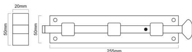
SB-5111-10"
