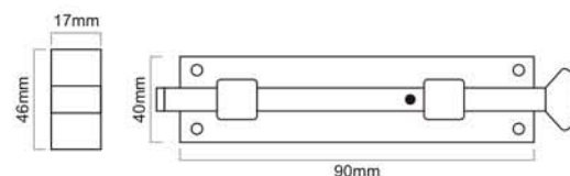
SB-5111-4"
